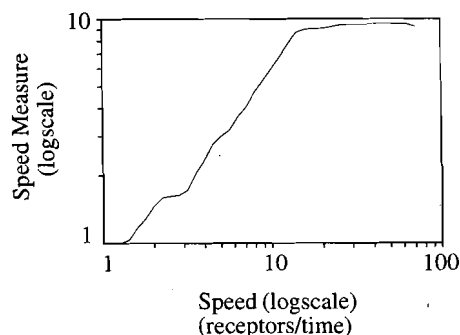
Fig. 4. Simulated speed measure as a function of input speed. The speed measure is obtained from a weighted sum of activities at all scales at the final network level (after the inter-scale competition). The speed measure increases approximately linearly with input speed until it saturates.
