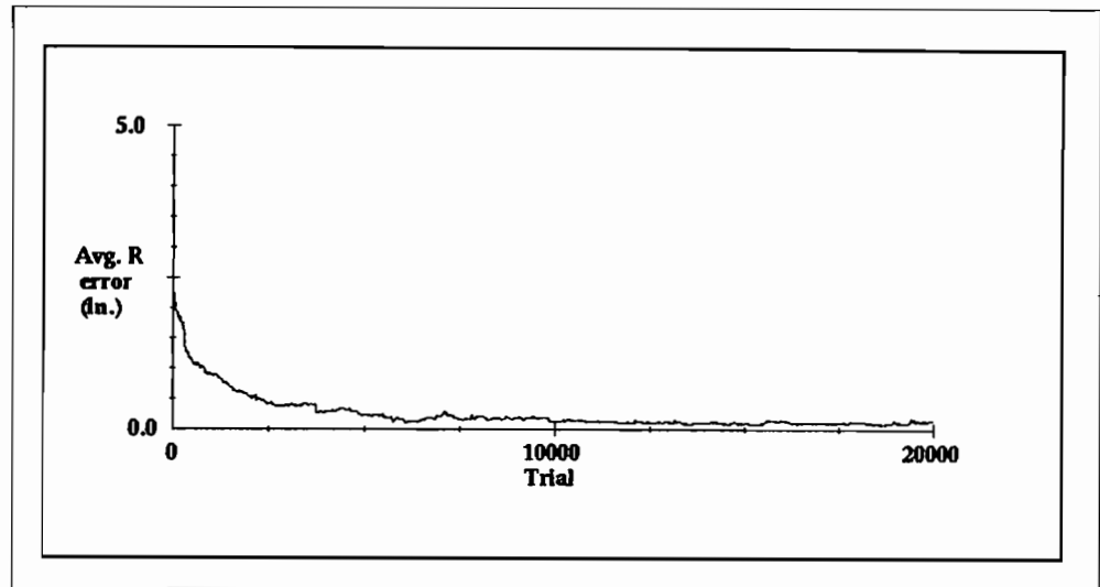
Figure 13. Average error of internal estimate of R_B during learning by the network of Figure 12.
