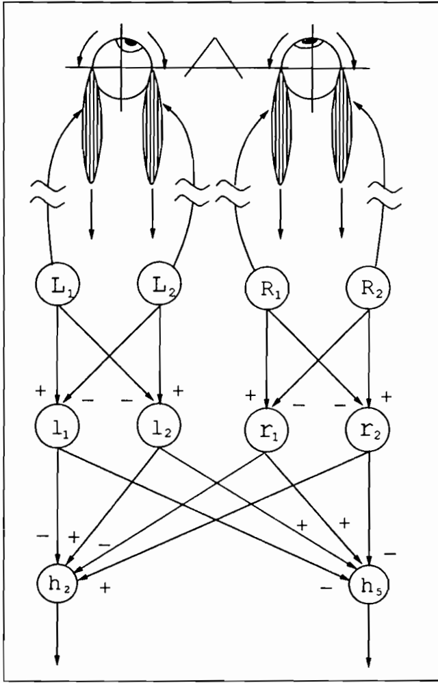
Figure 5. Opponent processing architecture for the calculation of the internal representation of gaze angle ( h_2 ) and vergence ( h_5 ). Signals L_1 , L_2 , R_1 , and R_2 are corollary discharges from the outflow movement cells that control eye position. The muscles are arranged in agonist-antagonist pairs. Stimulation by neuron L_2 causes a contraction of the left medial muscle, which rotates the left eyeball to the right. The activity of each pair of cells is normalized at cells l_1 , l_2 , r_1 , and r_2 .
