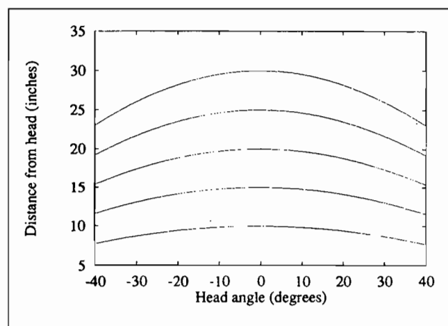
Figure 11. Actual positions of foveated objects that give rise to constant values of vergence (curved lines) for different head angles. Without the networks described in this section, an internal estimate of distance from the head for a fixed target based solely on vergence would suffer from the variability due to head position seen here. Human perception of distance is better than these isovergence-based estimates, particularly for nearer distances (Blank, 1978).
