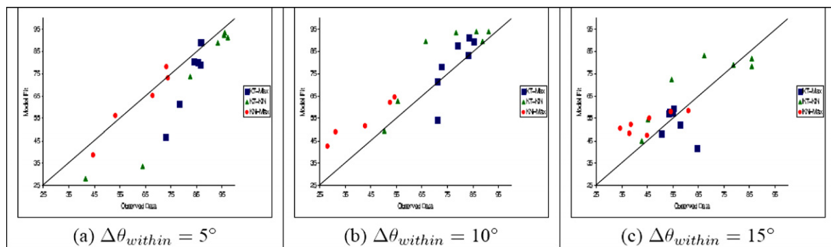
Fig. 8. Scatter plot of model output vs. data from Ben-Shahar and Zucker (2004) experiments. (a,b) The simulations for the cases \Delta\theta_{\text{within}} = 5^\circ and \Delta\theta_{\text{within}} = 10^\circ fit the observed data well. However, this fit is worse with \Delta\theta_{\text{within}} = 15^\circ in (c). See the test for an explanation of why this happens.
