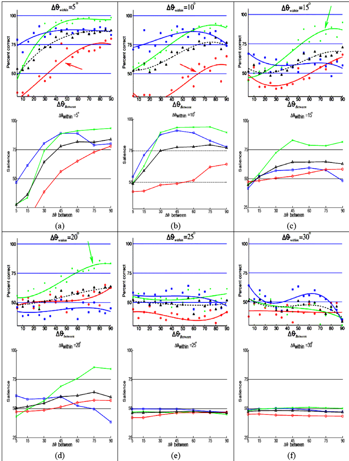
Fig. 3. Complete simulation results of the Ben-Shahar and Zucker (2004) experiments. Each panel shows detection accuracy curves for a specific image orientation gradient magnitude \Delta\theta_{\text{within}} as the boundary angular discontinuity amount \Delta\theta_{\text{between}} increases from 5^\circ to 90^\circ . Points marked by boxes (blue curves) belong to \Delta k_T = \max configurations, those marked by circles (red curves) are \Delta k_N = \max configurations, and those by crosses (green curves) are \Delta k_T = \Delta k_N configurations. Each of these configurations leads to a different configuration of texture bars. Average performance over all configurations is marked by triangles (black curves). For each panel, the top figure shows experimental data and the bottom panel shows dARTEx saliency outputs. See Section 3 for a complete description.
