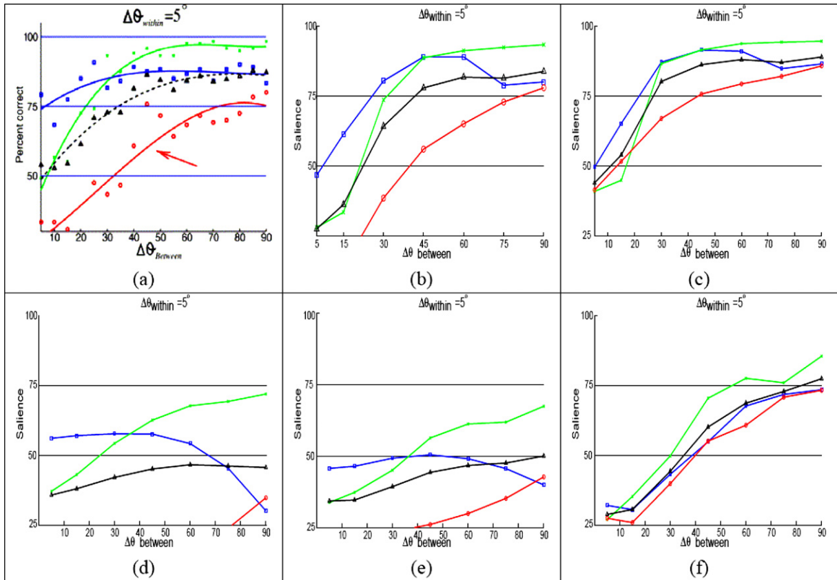
Fig. 6. Boundary attention and horizontal cooperative grouping are necessary for boundary processing. (a) Experimental data of Ben-Shahar and Zucker (2004). Green curve with crossed points: \Delta k_T = \Delta k_N , blue curve with boxed points: \Delta k_T = \max , red curve with circled points: \Delta k_N = \max and \Delta\theta_{\text{within}} = 5^\circ . Vertical axis: detection accuracy, horizontal axis: boundary discontinuity amount \Delta\theta_{\text{between}} . (b) With feedback and grouping operational and horizontal bipole orientations receiving the most weight with a Gaussian falloff in orientation, the data fit is very close to the observed results. (c) Same as part b, but with the same weight applied to all bipole orientations. (d) With no boundary-based attention modulating the LGN, the saliency actually drops at high \Delta\theta_{\text{between}} and \Delta k_T = \max due to the lack of boundary amplification that enable bipole grouping in horizontal orientation. (e) Bipole grouping disabled, and the V2 competitive stage outputs constitute feedback to LGN. Boundary saliency does not increase with increasing \Delta\theta_{\text{between}} for \Delta k_T = \max due to lack of boundary amplification by bipole grouping. (f) Same as (e) but with all orientations added with equal weight. Crossover of saliency curves vanishes. This output is very similar to the predicted output of the Filter–Rectifier–Filter model containing two stages of filters with intermediate point-wise nonlinearity.
